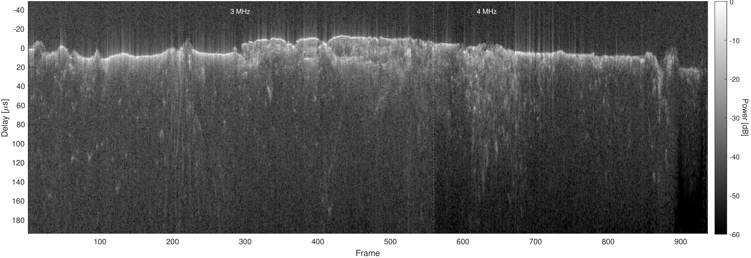
Orbit 8698, Optimized, No Window, Channel 2
