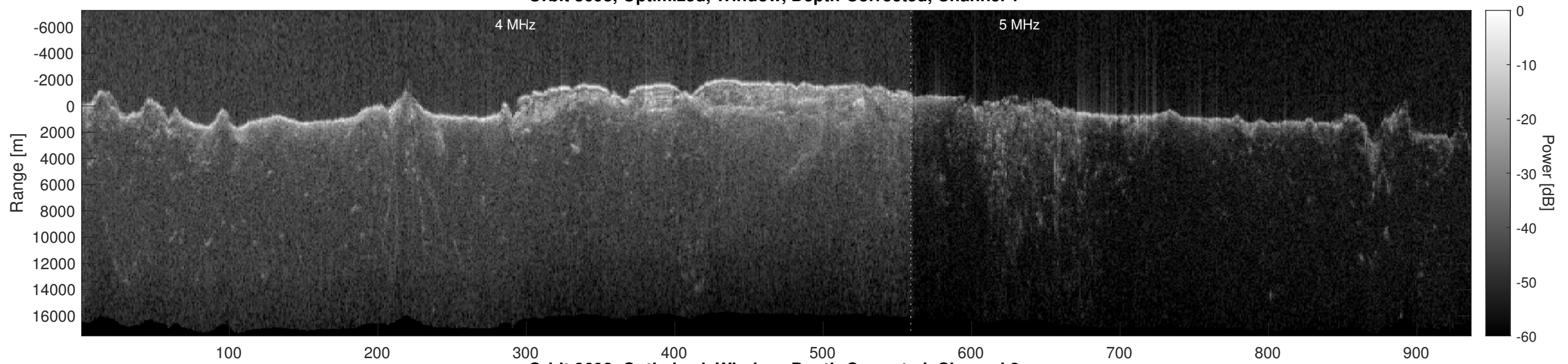
Orbit 8698, Optimized, Window, Depth-Corrected, Channel 2
