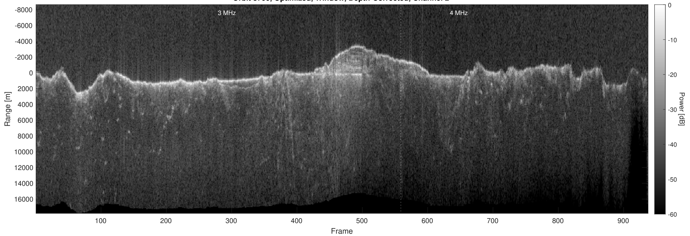
Orbit 8700, Optimized, Window, Depth-Corrected, Channel 2
