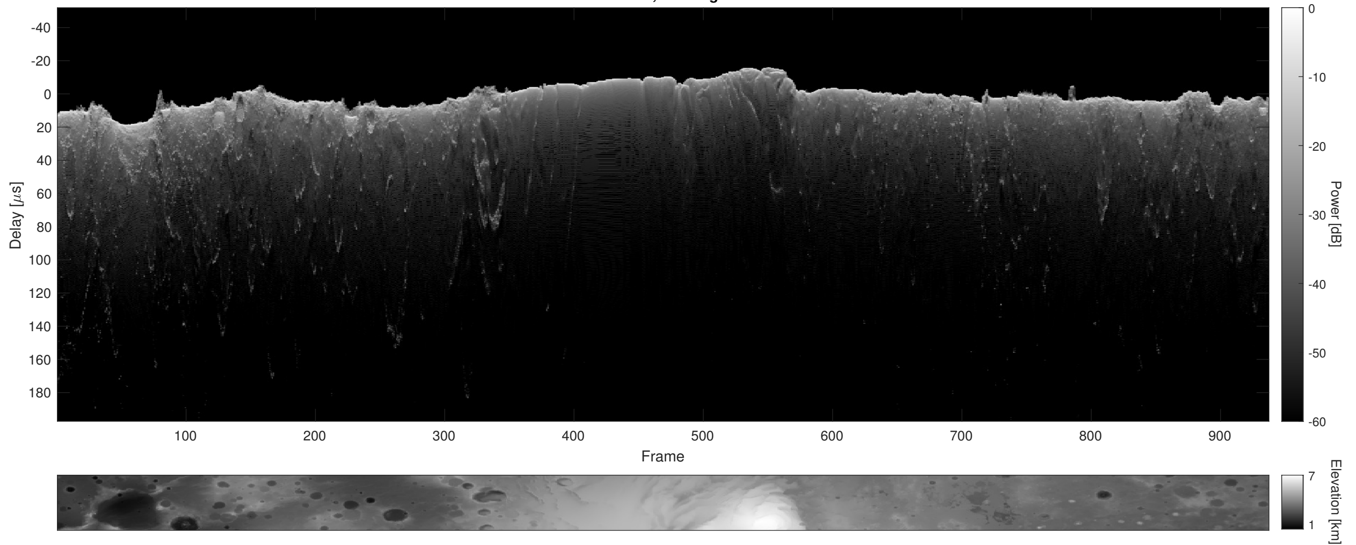
Orbit 8701, Cluttergram
