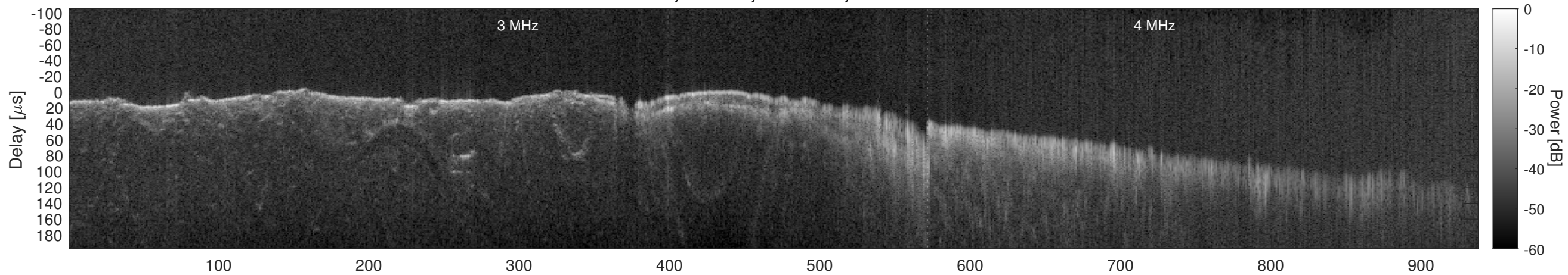
Orbit 8701, Window, Channel 2, Chapman
