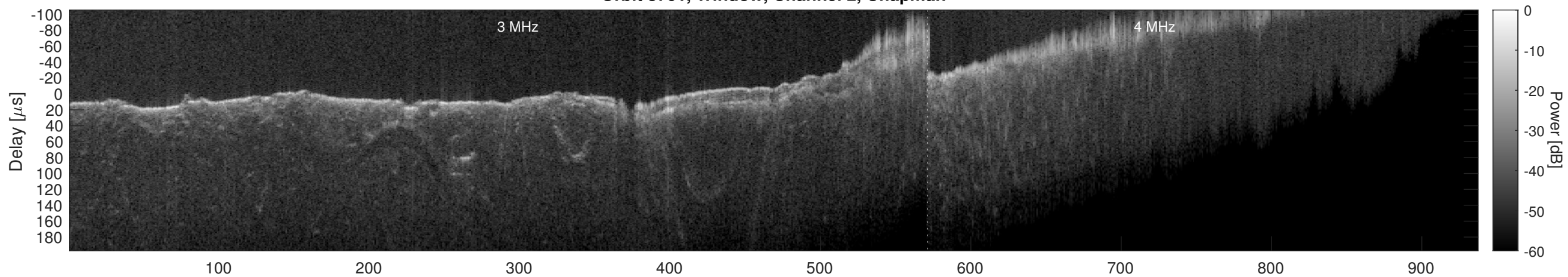
Orbit 8701, Window, Channel 2, Optimized
