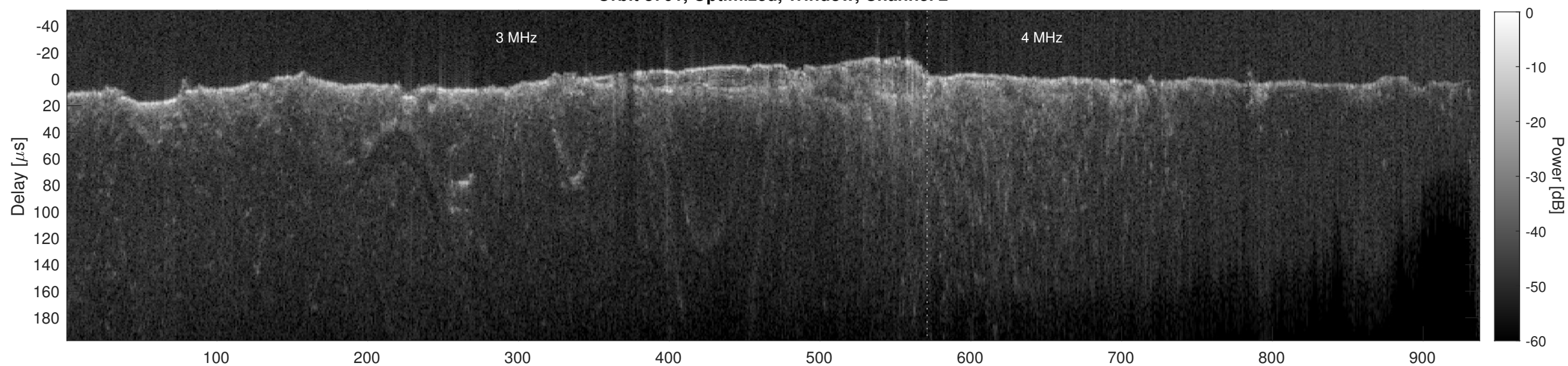
Orbit 8701, Cluttergram
