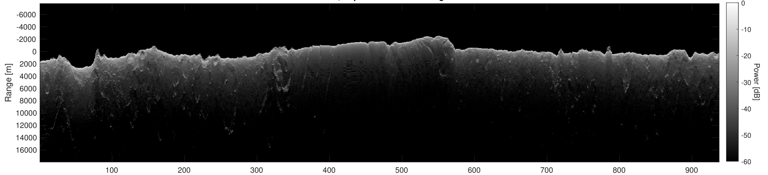
Orbit 8701, Depth-Corrected Cluttergram
