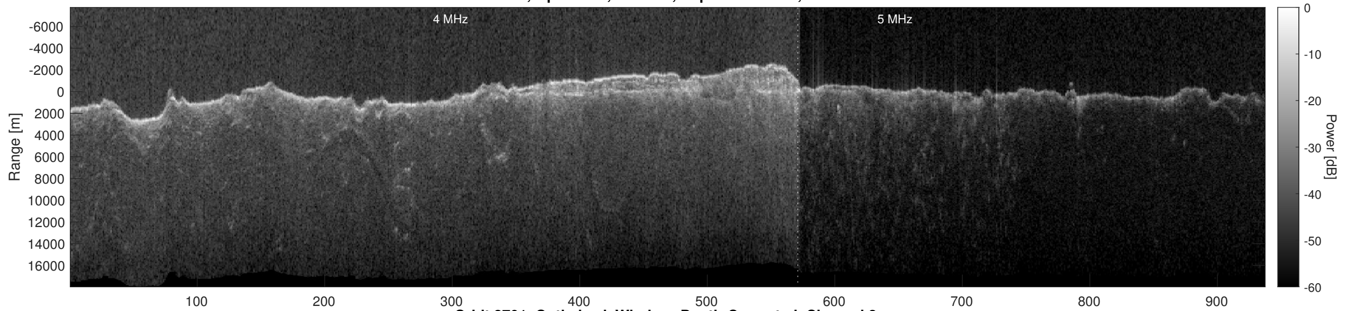
Orbit 8701, Optimized, Window, Depth-Corrected, Channel 2
