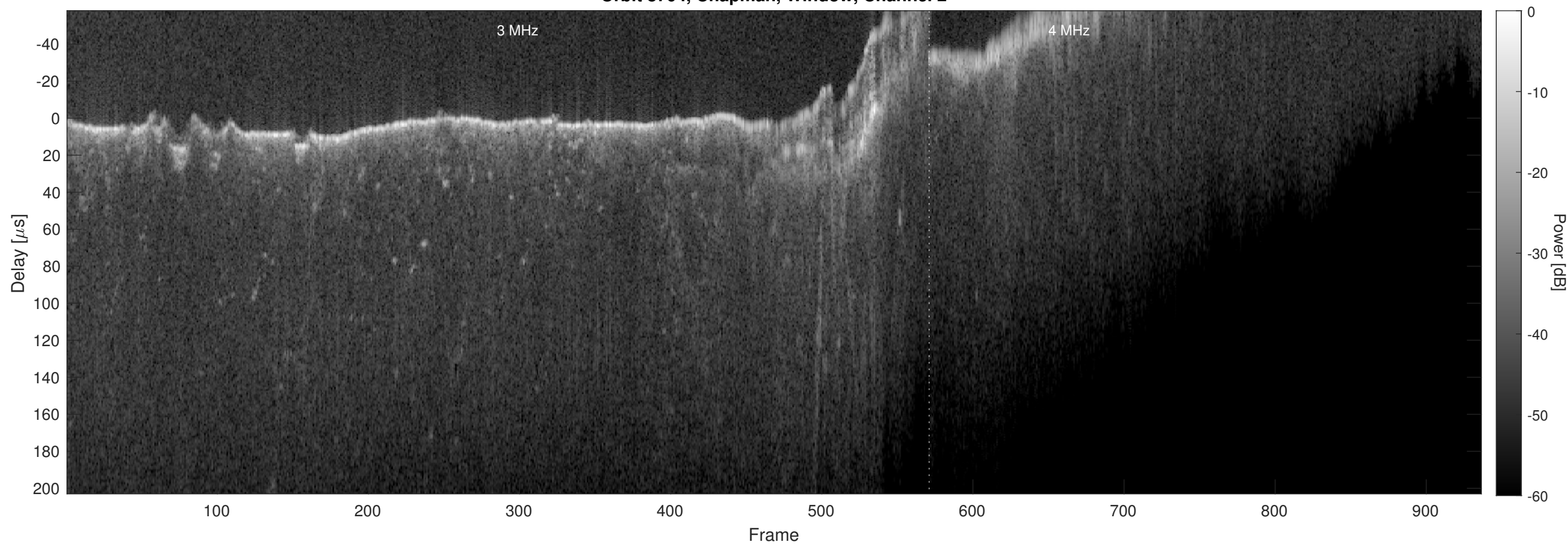
Orbit 8704, Chapman, Window, Channel 2
