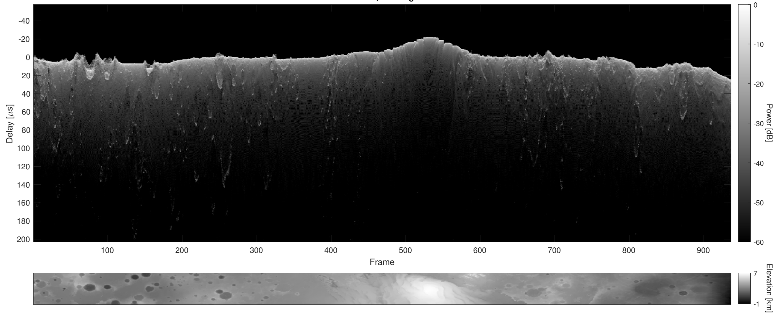
Orbit 8704, Cluttergram
