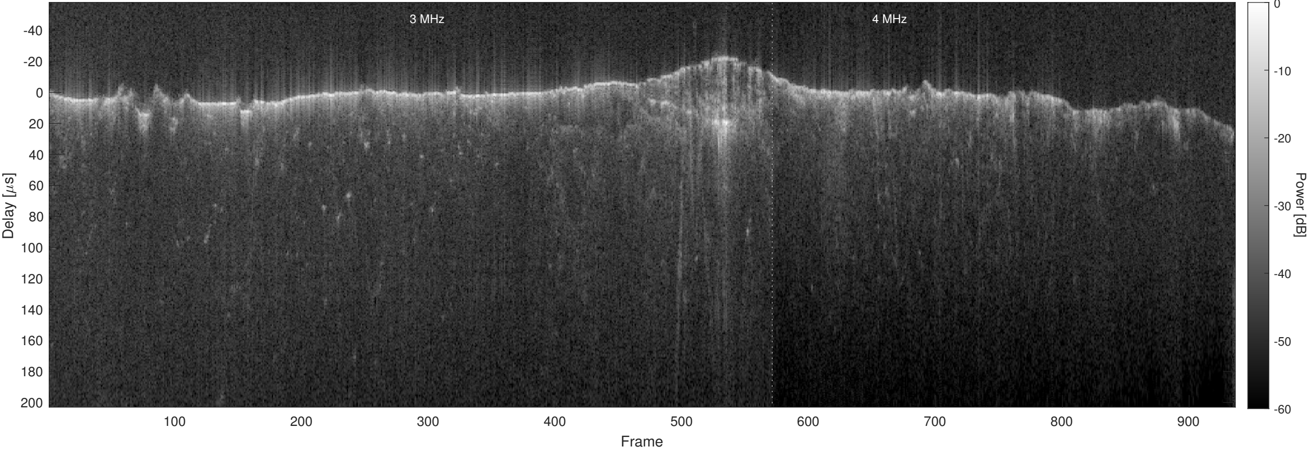
Orbit 8704, Optimized, No Window, Channel 2
