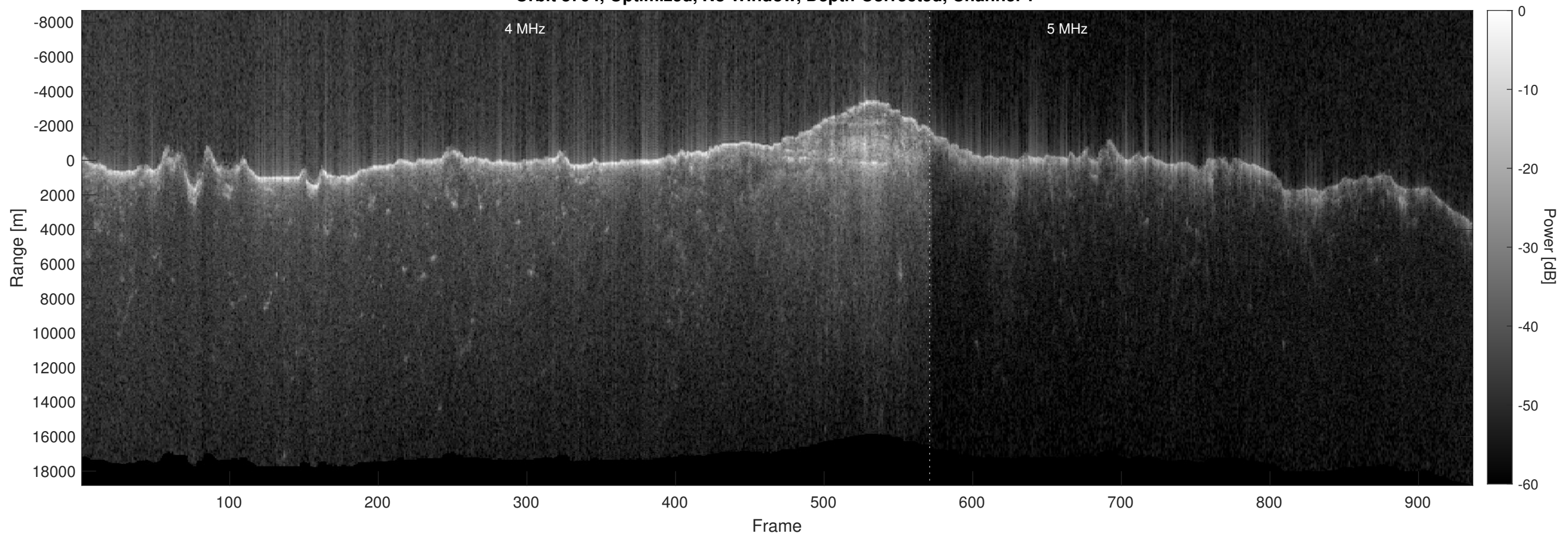
Orbit 8704, Optimized, No Window, Depth-Corrected, Channel 2
