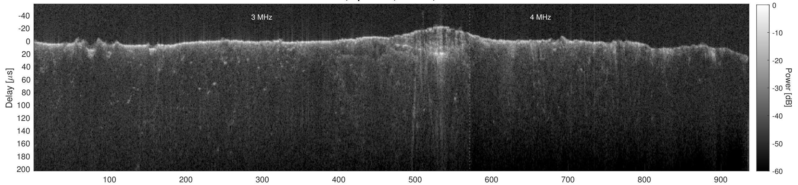
Orbit 8704, Cluttergram
