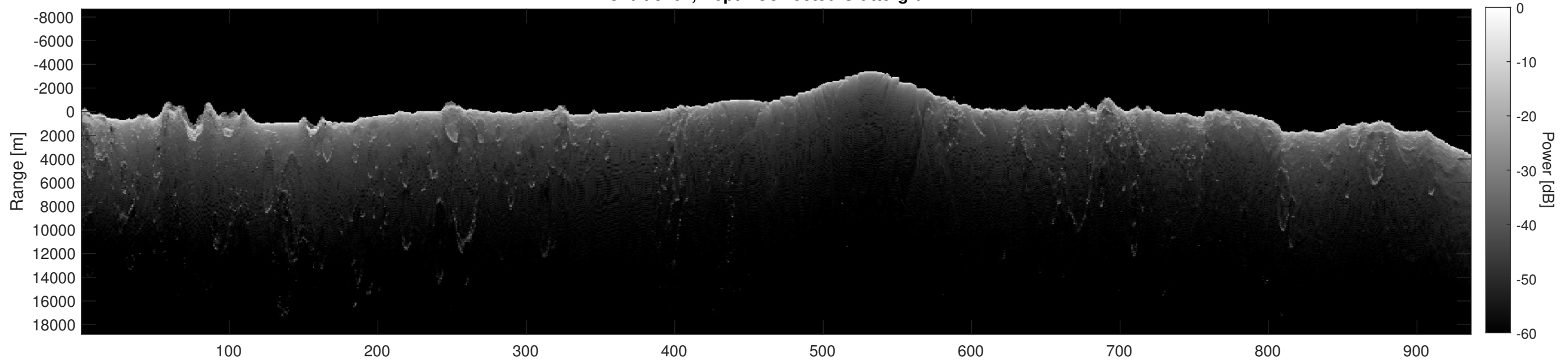
Orbit 8704, Depth-Corrected Cluttergram
