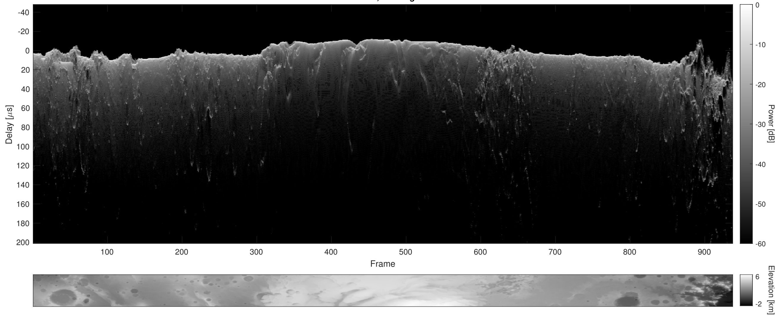
Orbit 8705, Cluttergram
