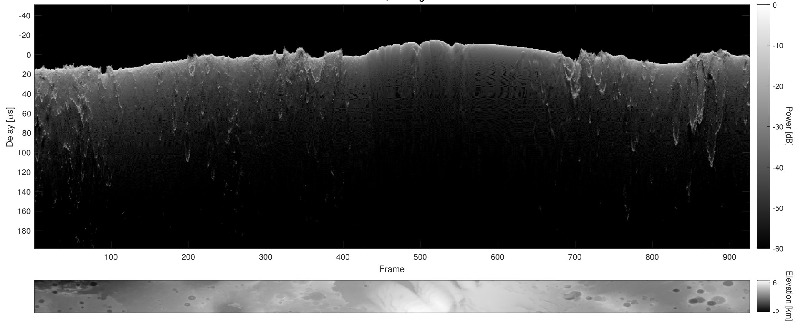
Orbit 8706, Cluttergram
