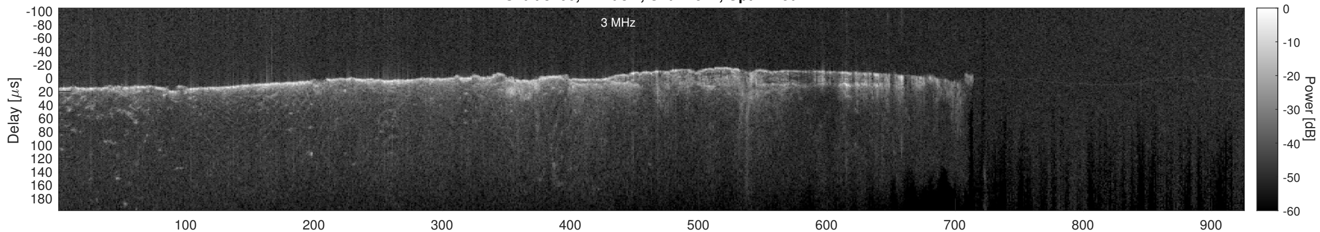
Orbit 8706, Cluttergram
