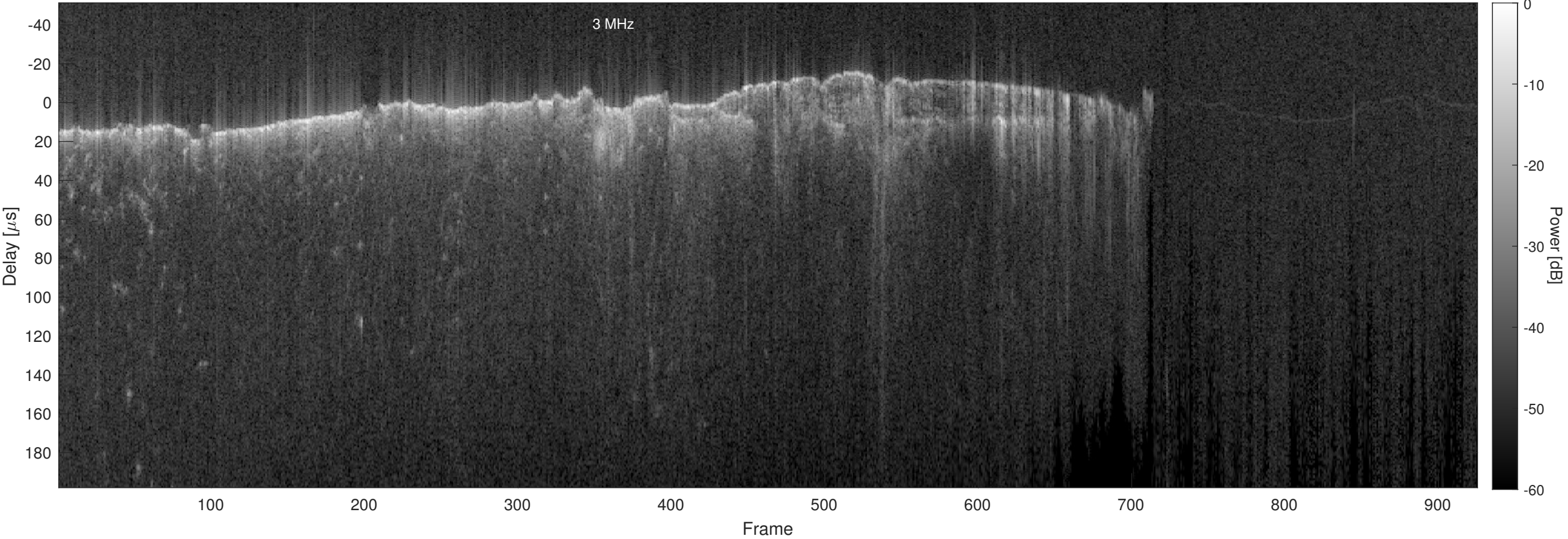
Orbit 8706, Optimized, No Window, Channel 2
