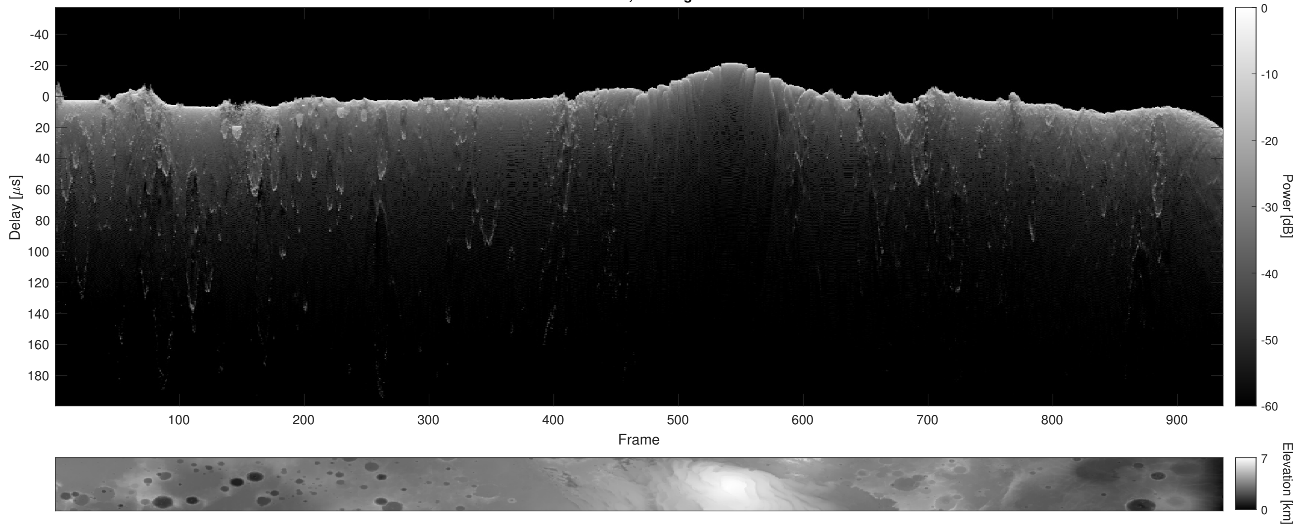
Orbit 8711, Cluttergram
