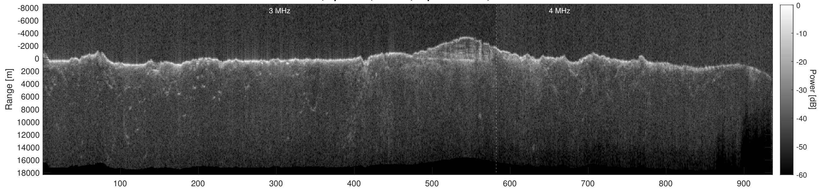
Orbit 8711, Depth-Corrected Cluttergram
