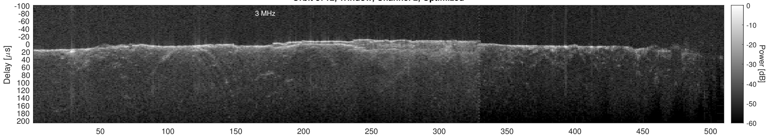
Orbit 8712, Cluttergram
