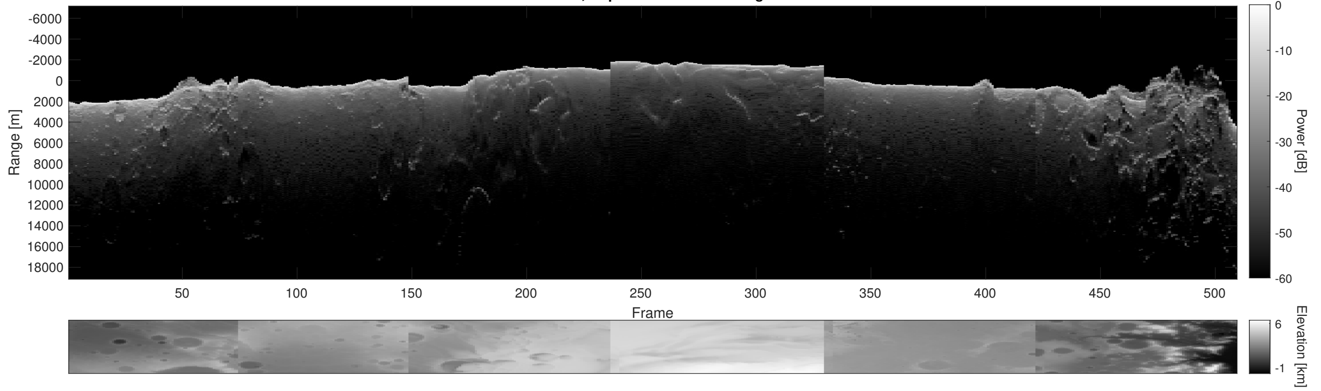
Orbit 8712, Depth-Corrected Cluttergram
