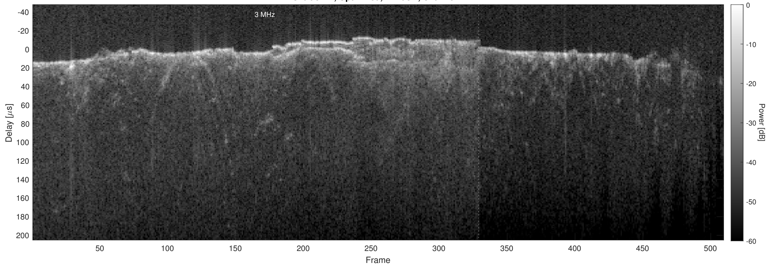
Orbit 8712, Optimized, Window, Channel 2
