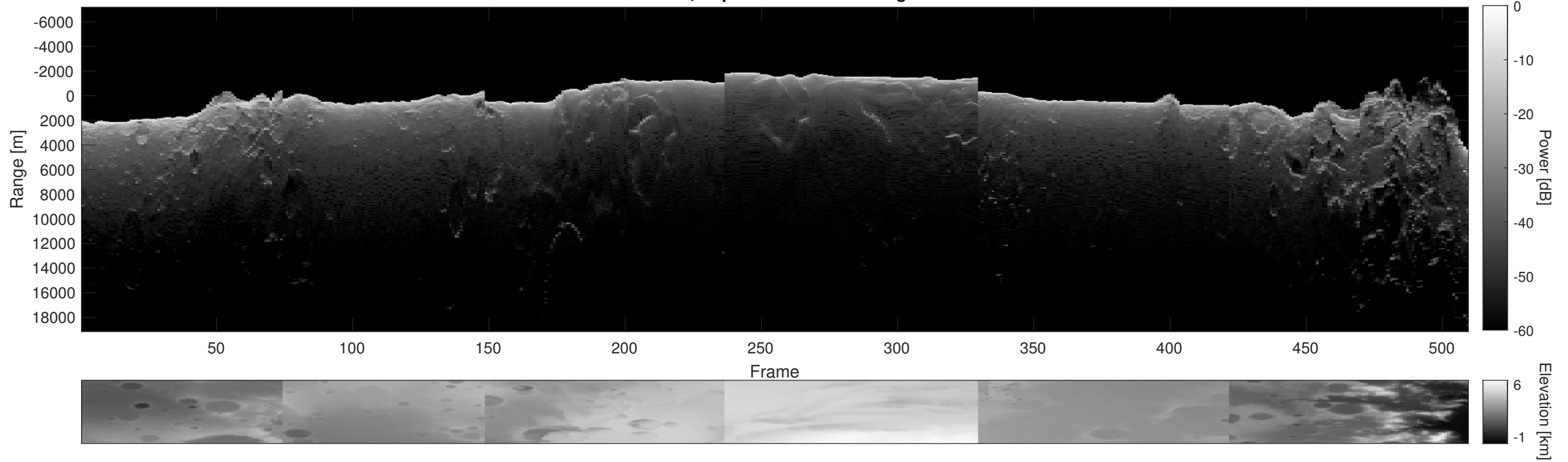
Orbit 8712, Depth-Corrected Cluttergram
