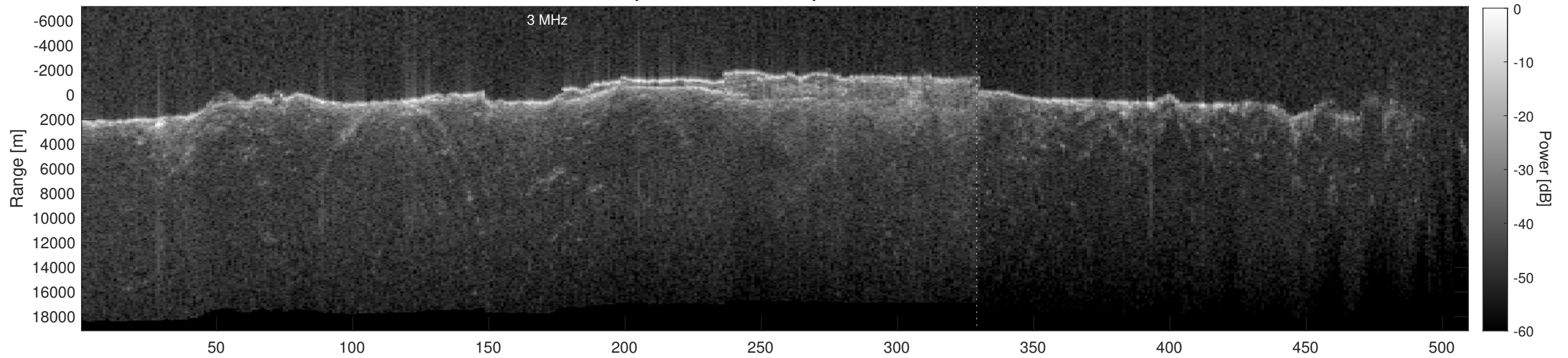
Orbit 8712, Depth-Corrected Cluttergram
