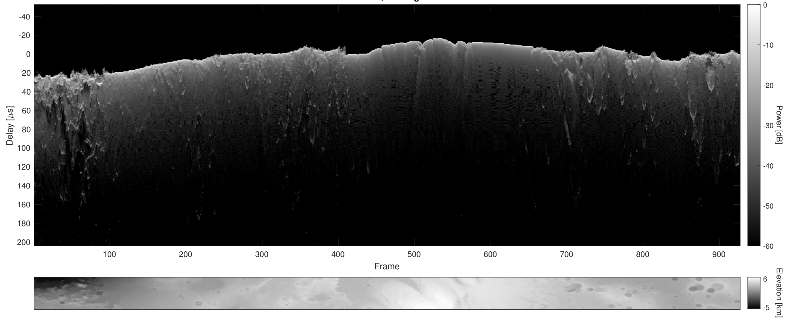
Orbit 8713, Cluttergram
