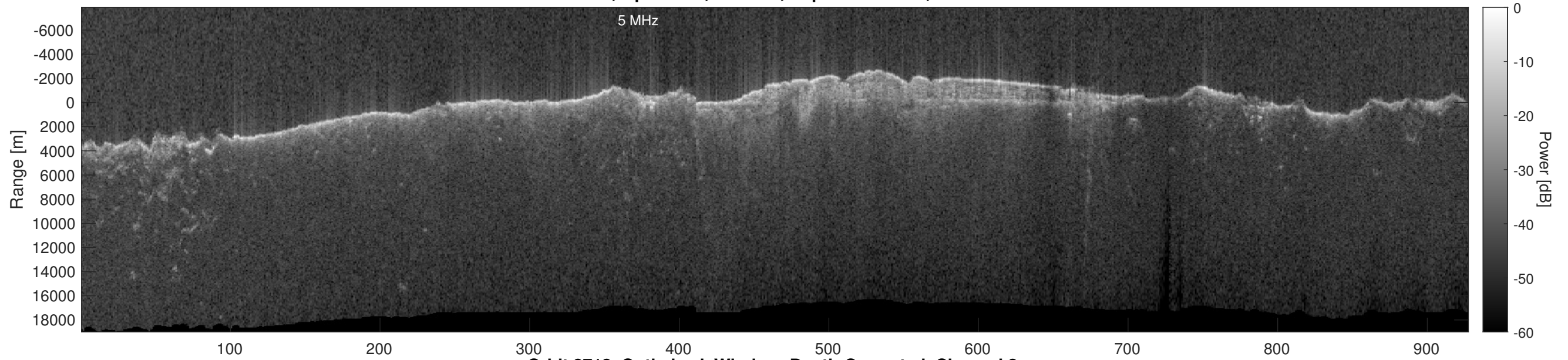
Orbit 8713, Optimized, Window, Depth-Corrected, Channel 2
