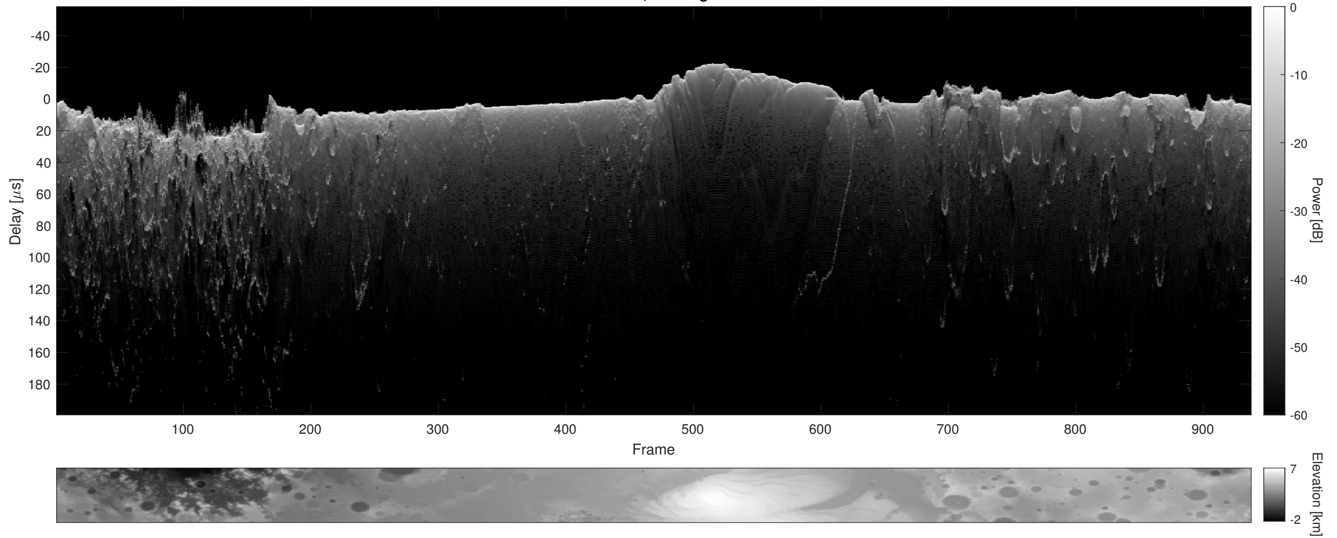
Orbit 8714, Cluttergram
