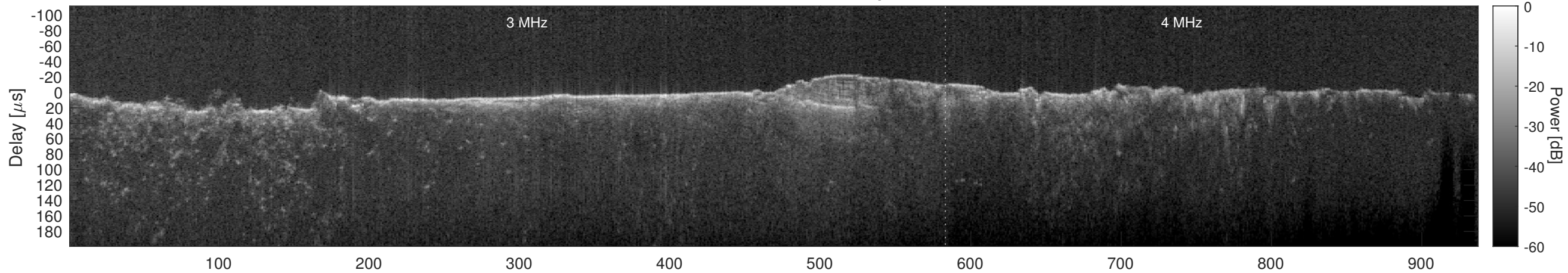
Orbit 8714, Cluttergram
