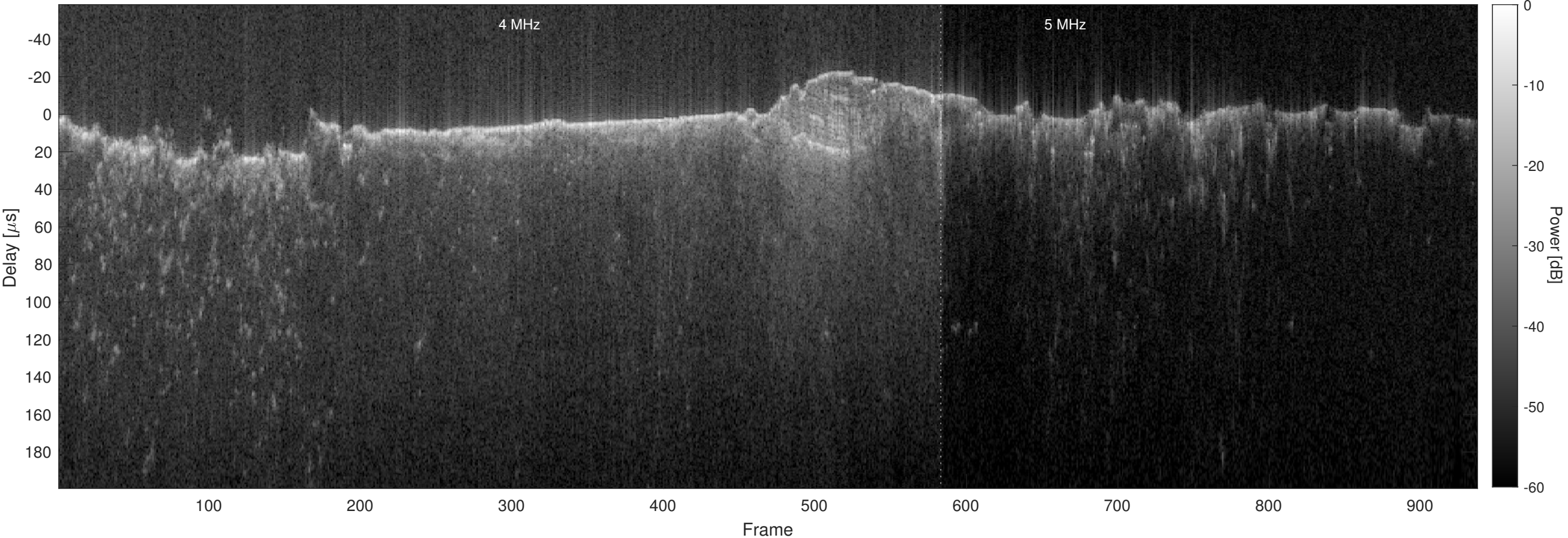
Orbit 8714, Optimized, No Window, Channel 2
