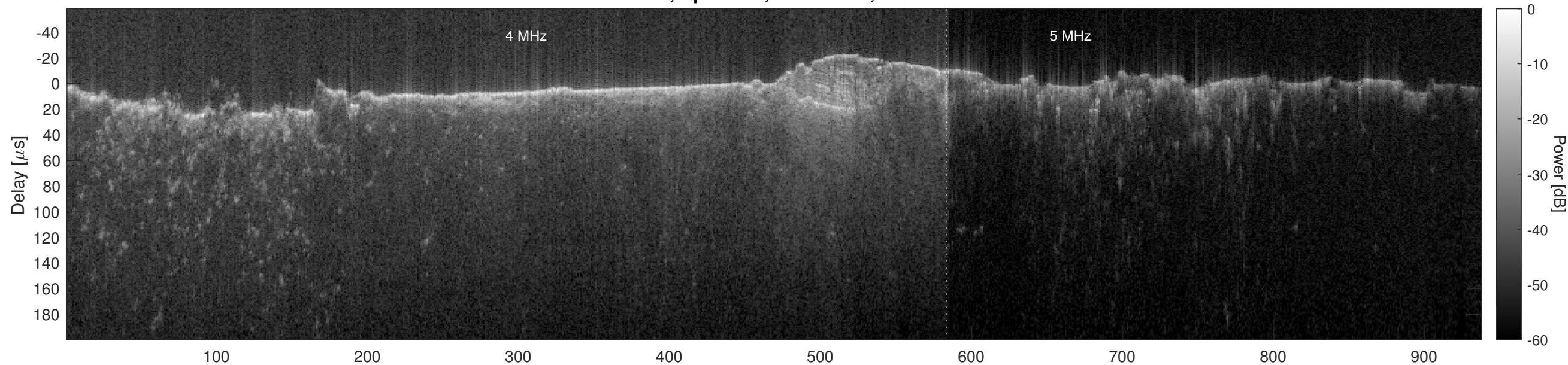
Orbit 8714, Optimized, No Window, Channel 2
