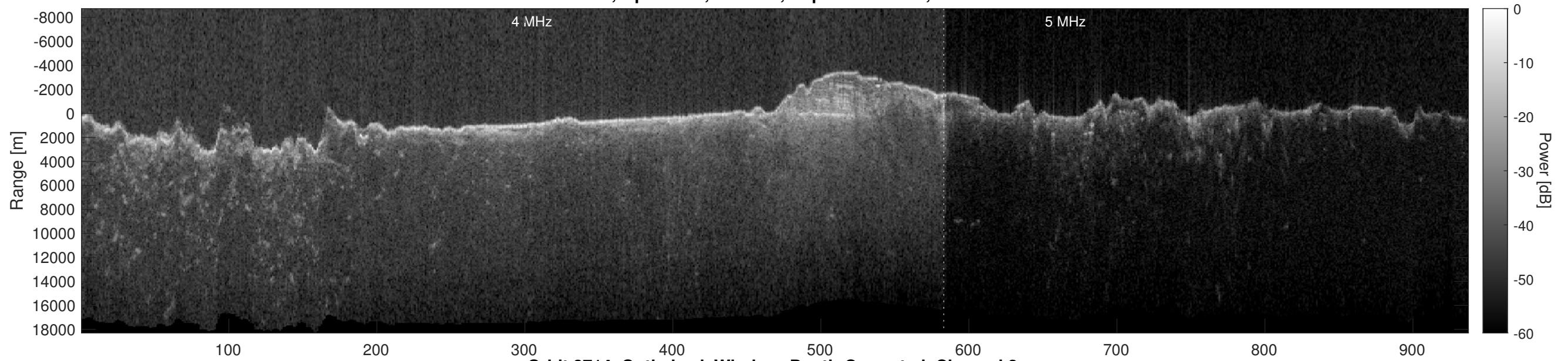
Orbit 8714, Optimized, Window, Depth-Corrected, Channel 2
