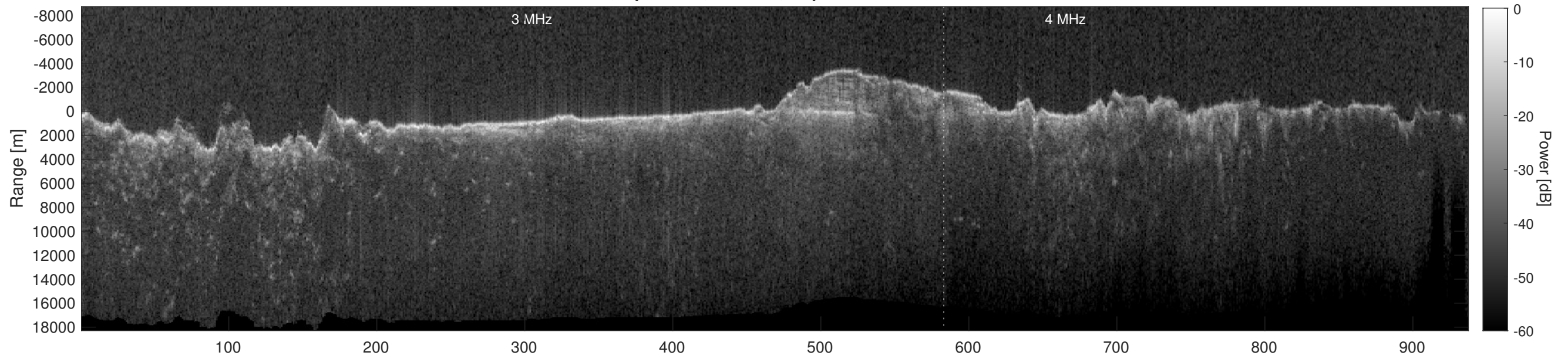
Orbit 8714, Depth-Corrected Cluttergram
