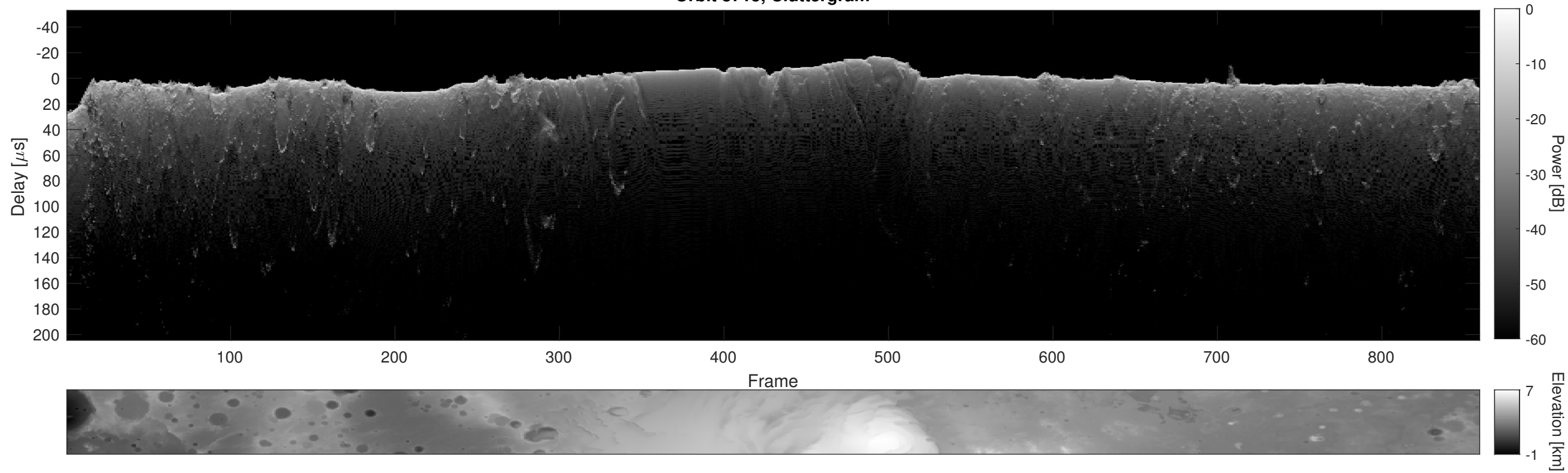
Orbit 8715, Cluttergram
