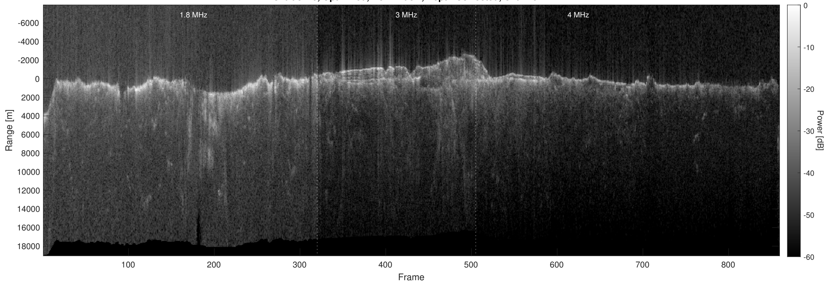
Orbit 8715, Optimized, No Window, Depth-Corrected, Channel 2
