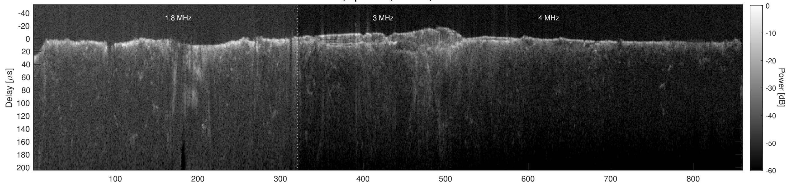
Orbit 8715, Cluttergram
