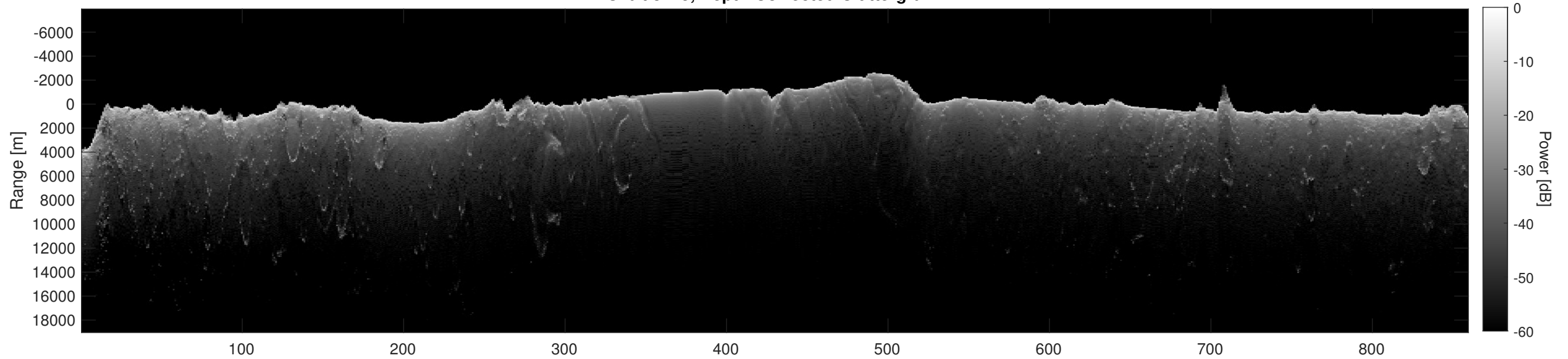
Orbit 8715, Depth-Corrected Cluttergram
