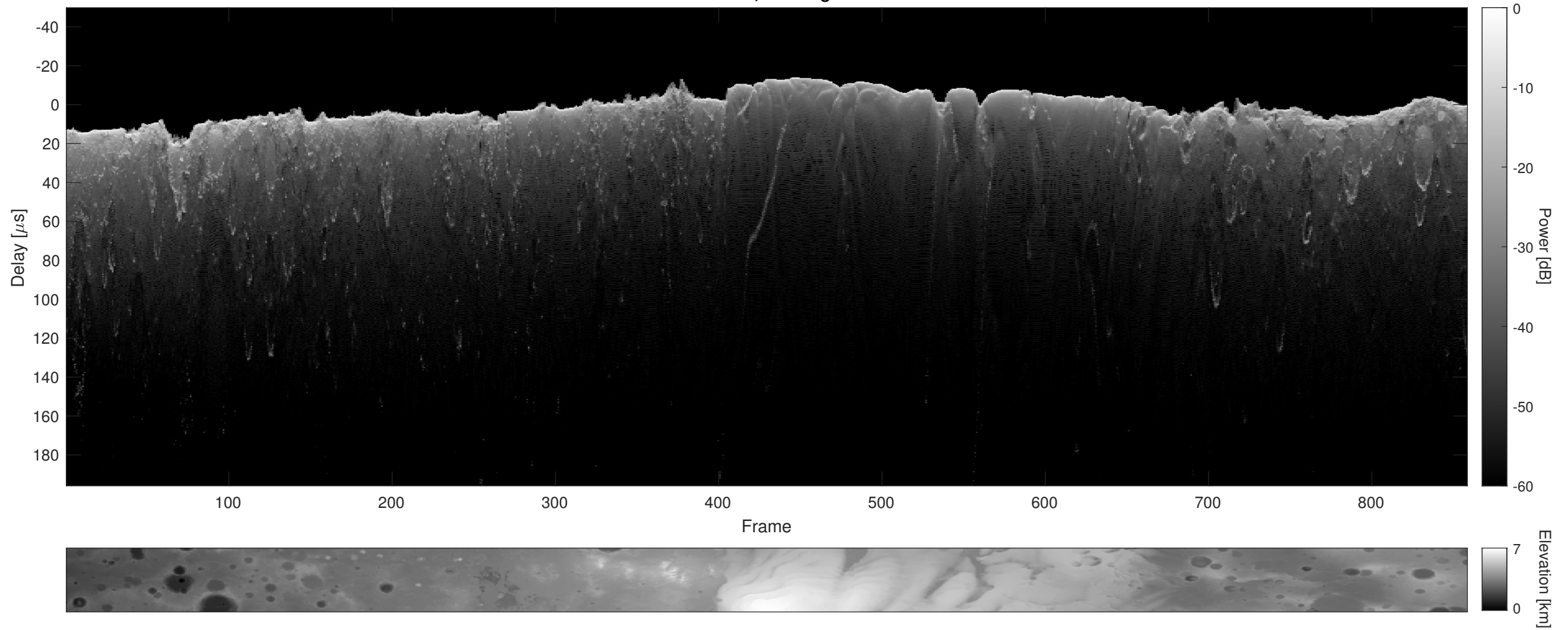
Orbit 8717, Cluttergram
