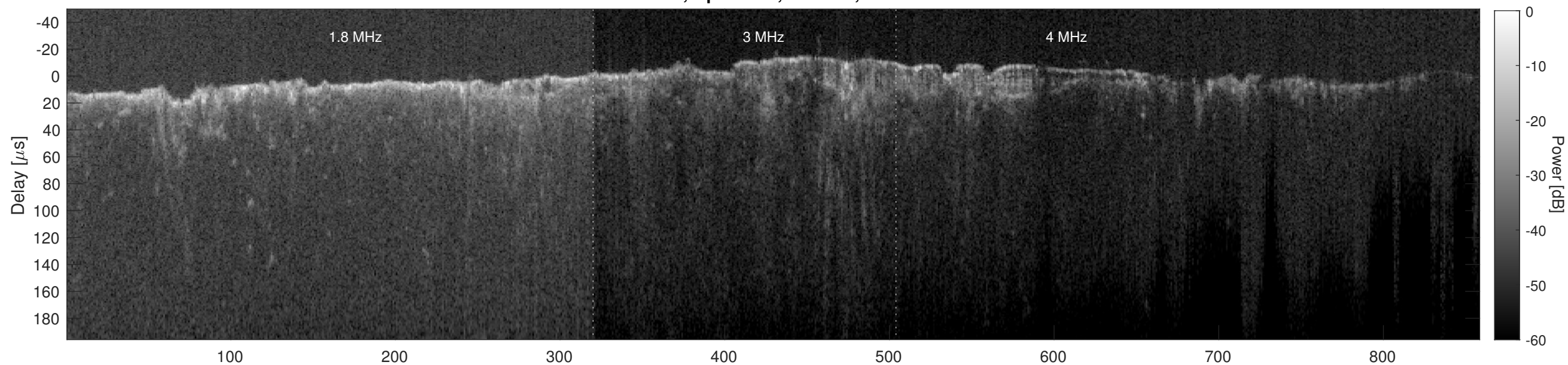
Orbit 8717, Cluttergram
