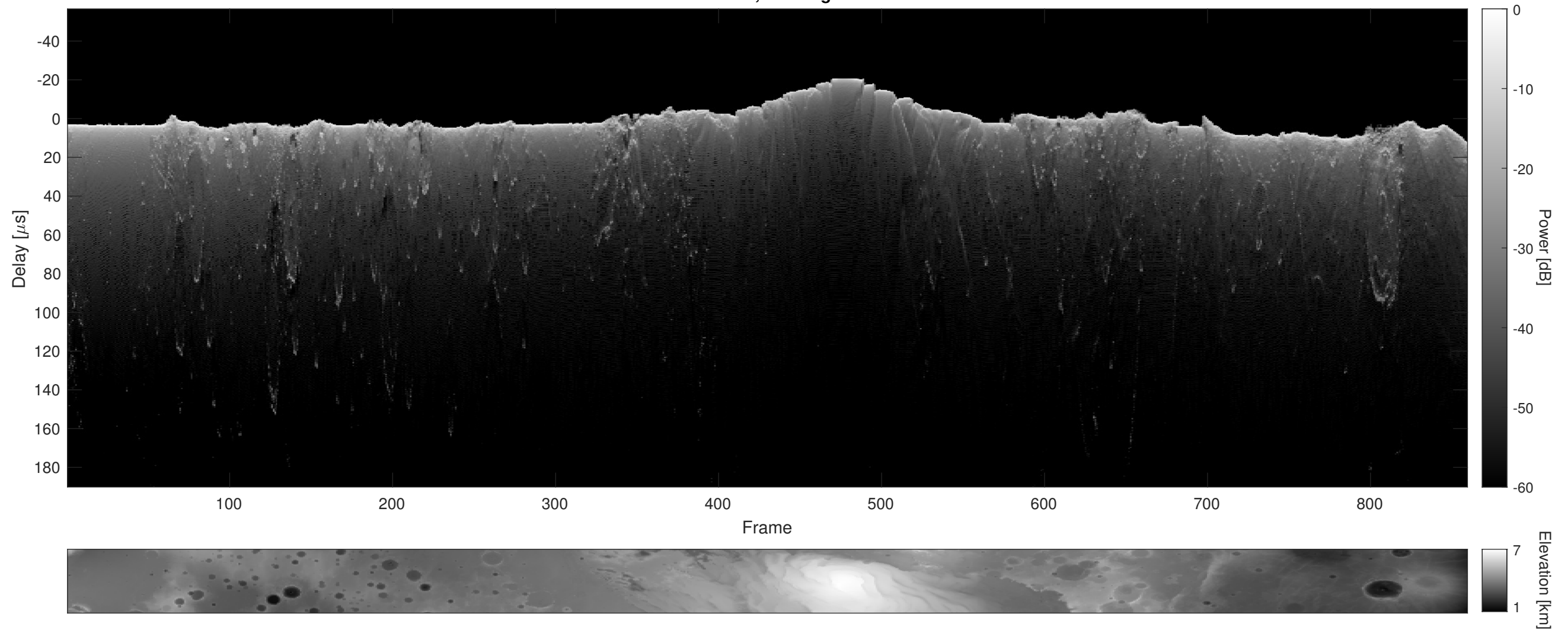
Orbit 8718, Cluttergram
