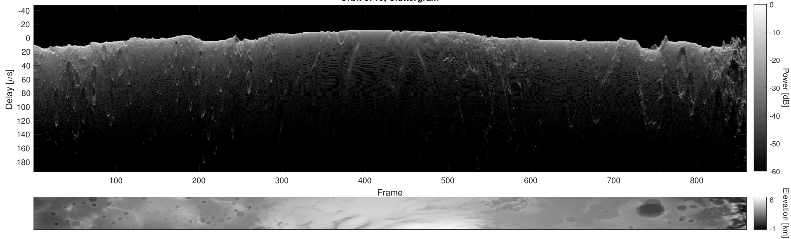
Orbit 8719, Cluttergram
