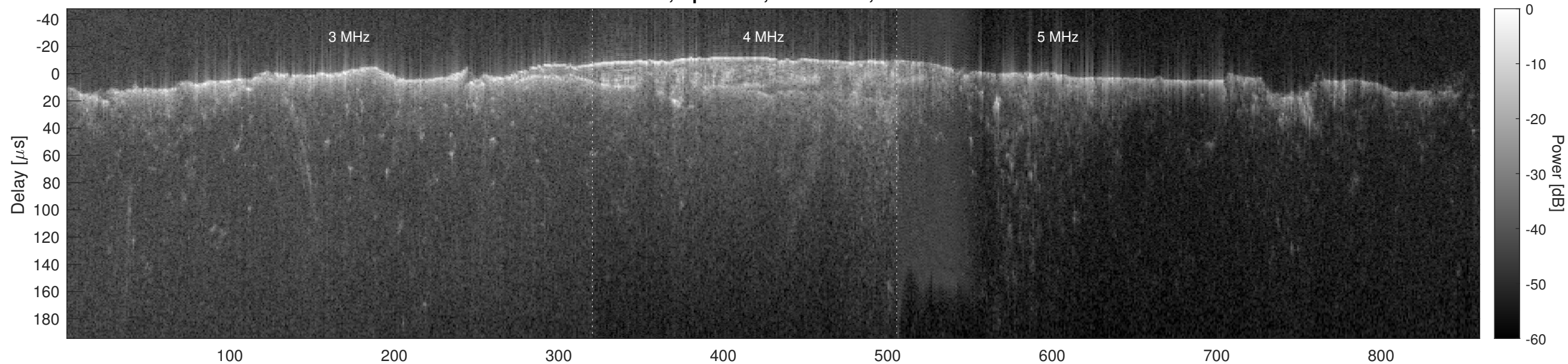
Orbit 8719, Optimized, No Window, Channel 2
