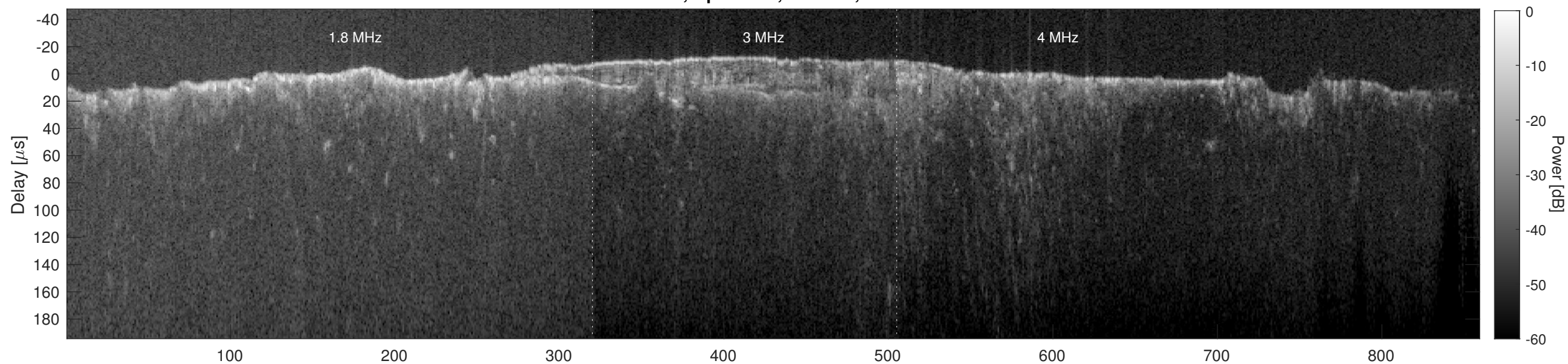
Orbit 8719, Cluttergram
