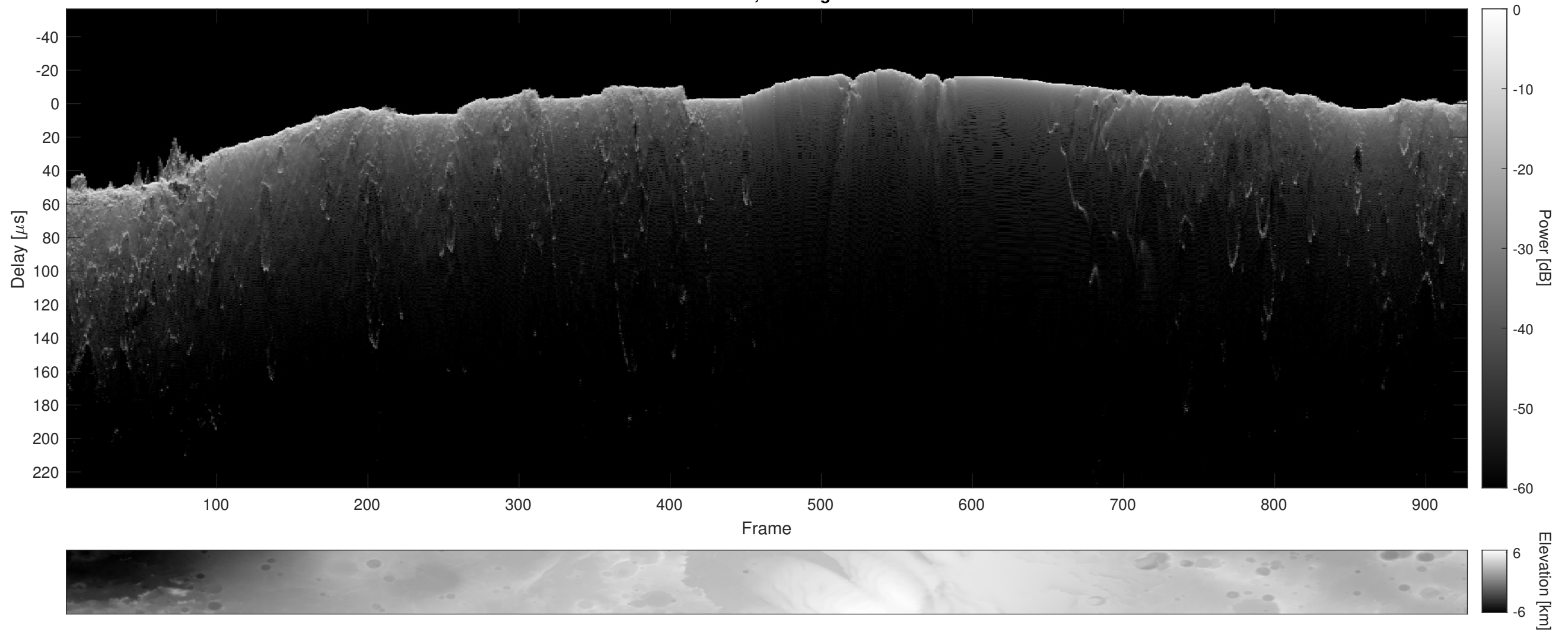
Orbit 8720, Cluttergram
