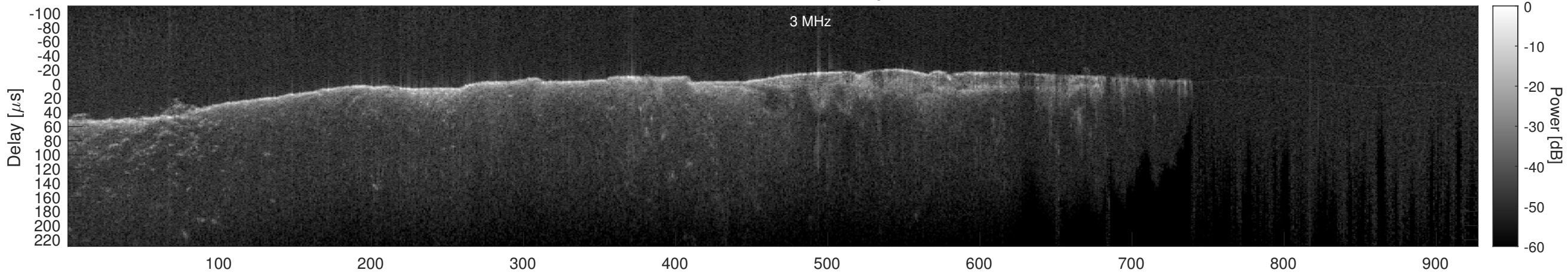
Orbit 8720, Cluttergram
