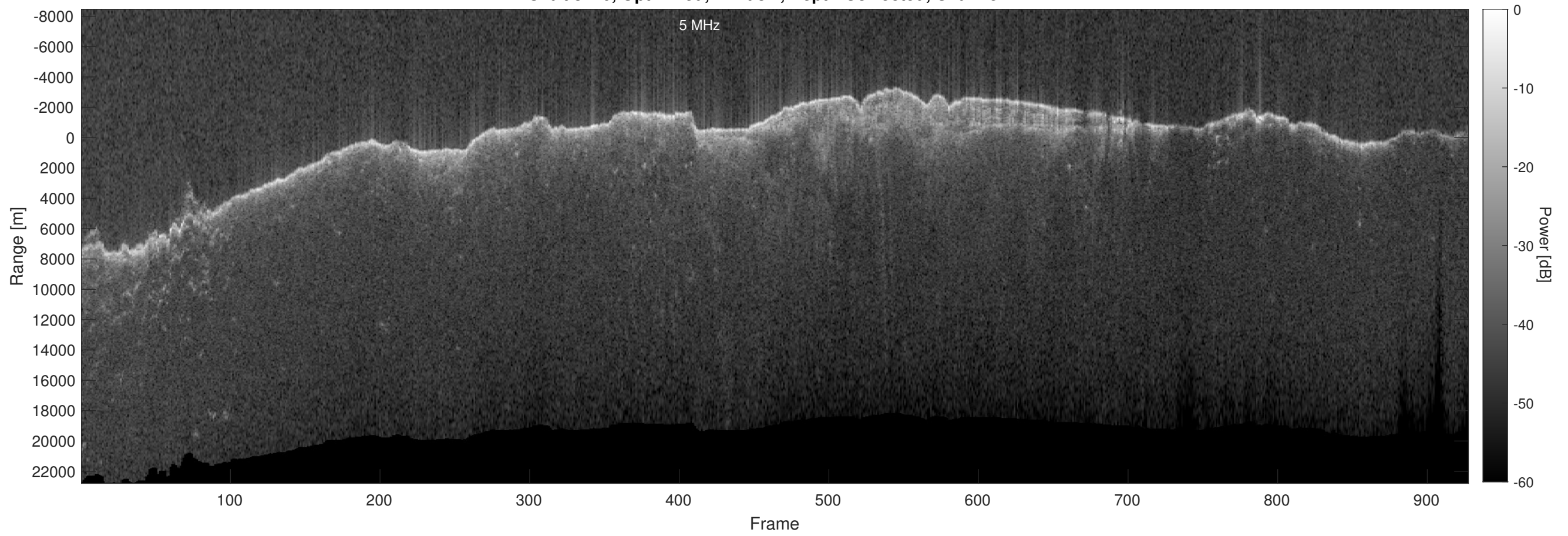
Orbit 8720, Optimized, Window, Depth-Corrected, Channel 2
