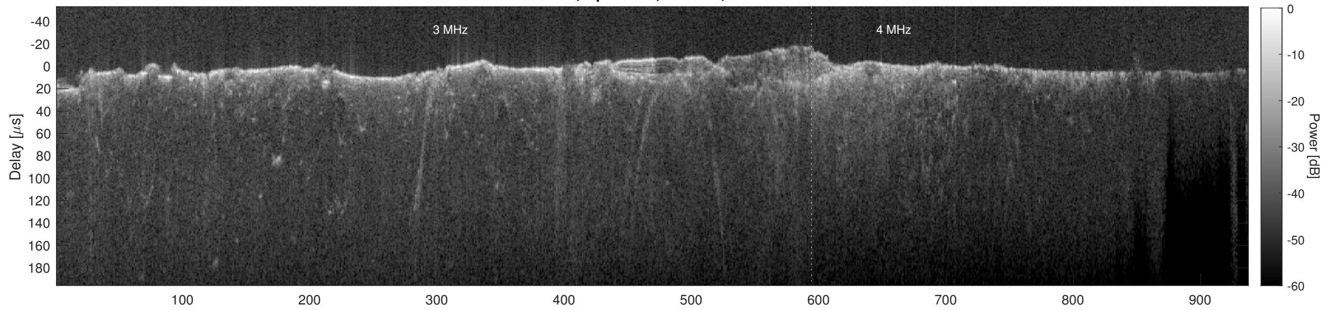
Orbit 8722, Cluttergram
