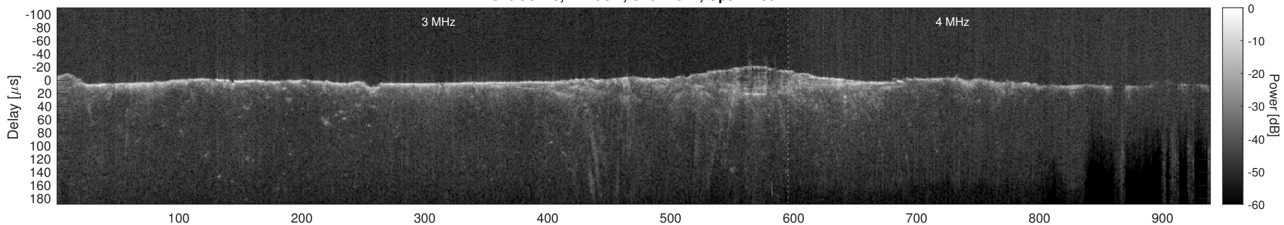
Orbit 8725, Cluttergram
