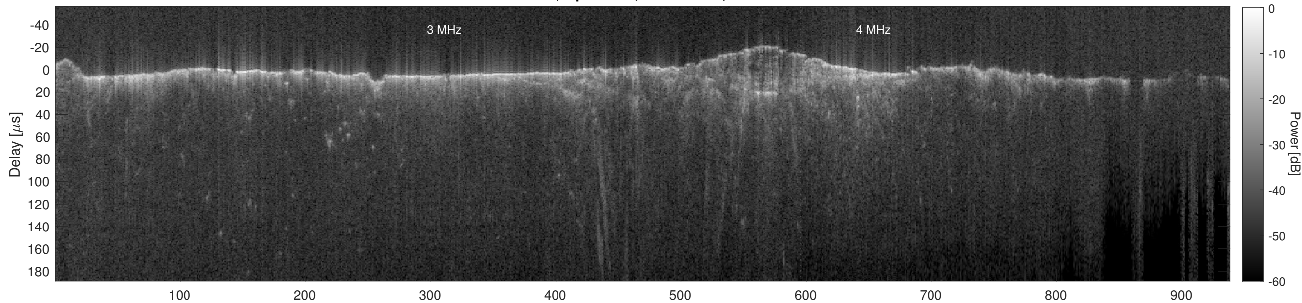
Orbit 8725, Cluttergram
