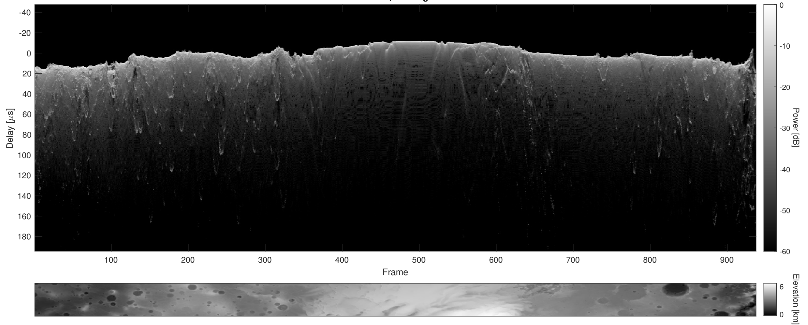
Orbit 8726, Cluttergram
