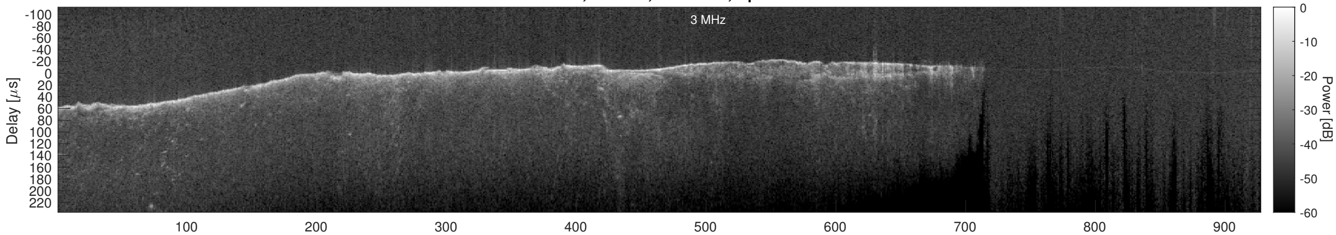
Orbit 8727, Cluttergram
