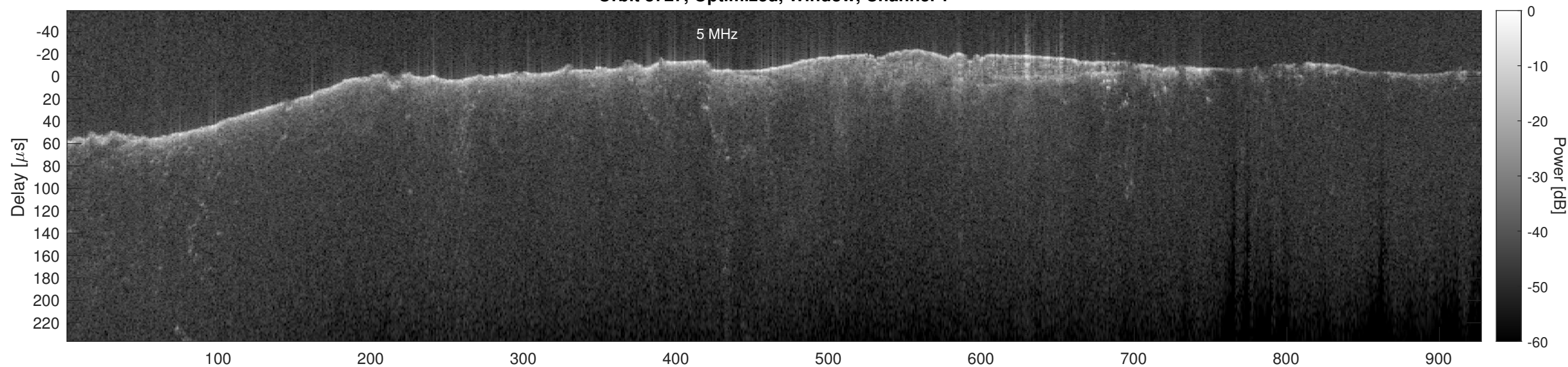
Orbit 8727, Optimized, Window, Channel 2
