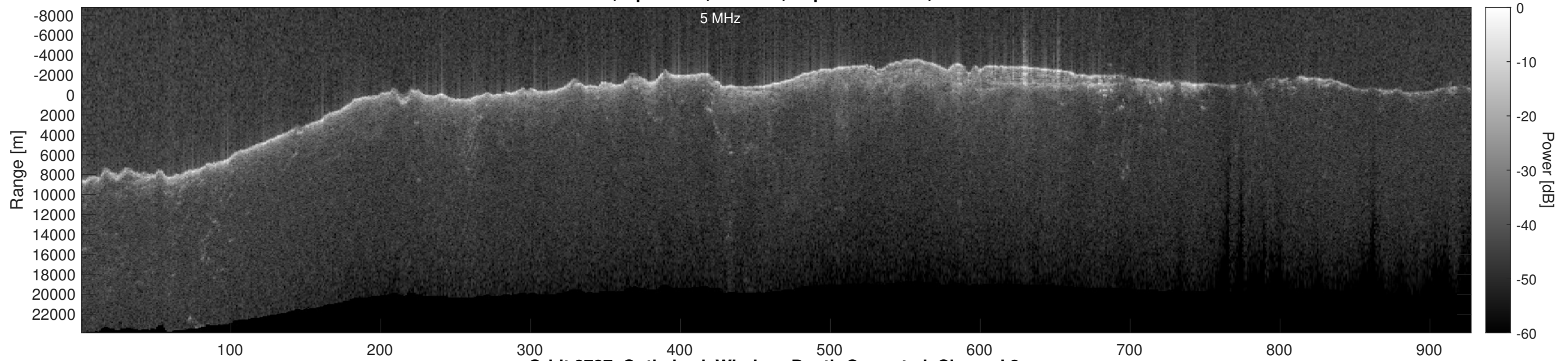
Orbit 8727, Optimized, Window, Depth-Corrected, Channel 2
