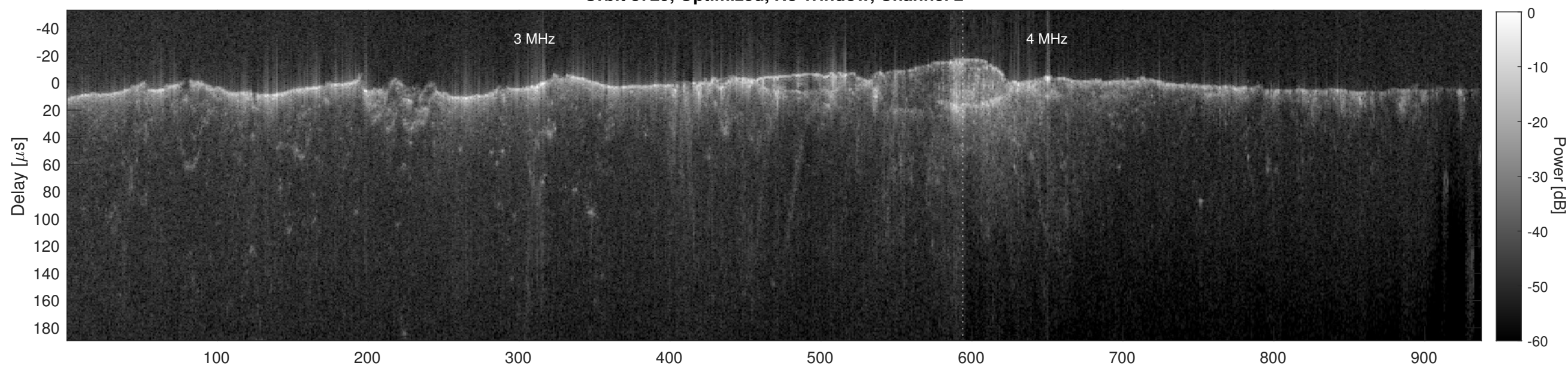
Orbit 8729, Cluttergram
